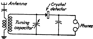
Circuit of typical crystal set.
